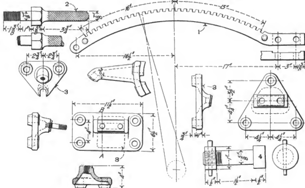
Section A-B. Figs. 1976-1988. Details of Reverse Lever Quadrant and Brackets for Atlantic (4-4-2) Locomotive. Pennsylvania Railroad.
